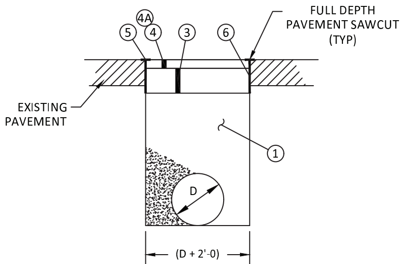
ASPHALT PAVEMENT REPAIR
