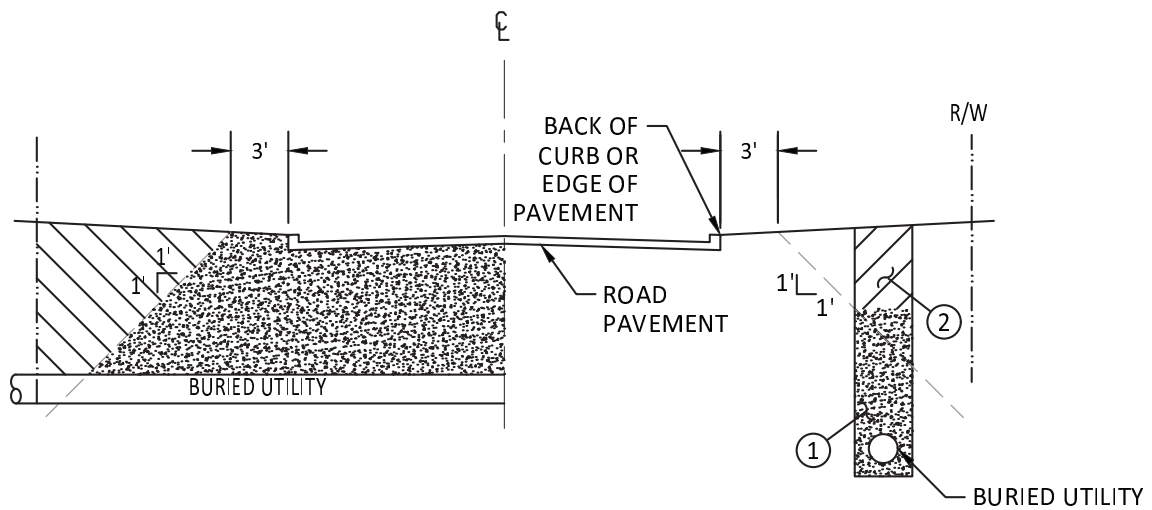
UTILITY TRENCHES WITHIN PAVEMENT INFLUENCE
