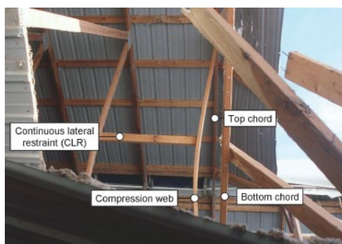
Figure 2: Shifting of the CLR enables the compression web to buckle out of the plane of the truss. All trusses to the right of the one labeled here failed in a progressive manner.
